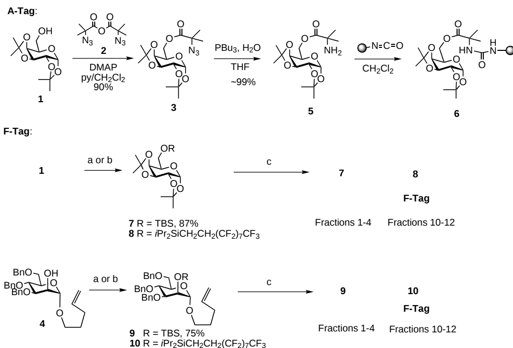
Scheme 2. Model monosaccharide synthesis and scavenging. a) 4 equiv (heptafluorodecyl)diisopropylsilyl triflate ( 11 ), 6 equiv 2,6-lutidine in \text{CH}_2\text{Cl}_2 at RT; b) 1.1 equiv TBSOTf, 2 equiv 2,6-lutidine in \text{CH}_2\text{Cl}_2 at RT; c) fluorosilyl silica gel ( \text{Si}(\text{CH}_2\text{CH}_2\text{C}_6\text{F}_5)_3 ), gradient of 80/20% \text{H}_2\text{O} to 100% MeOH. Bn = benzyl, DMAP = 4-dimethylaminopyridine, py = pyridine; TBS = t\text{BuMe}_2\text{Si} .
