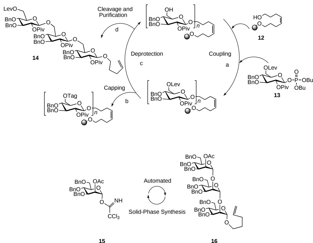
Scheme 3. Top: Synthesis of triglucoside 14 in a capping cycle. a) 5 equiv 13 , 5 equiv TMSOTf, -15^\circ\text{C} , \text{CH}_2\text{Cl}_2 ; b) A-Tag: 5 equiv 2 , DMAP, py/ \text{CH}_2\text{Cl}_2 ; F-Tag: 5 equiv 11 , 2,6-lutidine; c) \text{NH}_2\text{NH}_2 , 15^\circ\text{C} , py/AcOH; d) (1) ethylene, 0.2 equiv Grubbs' catalyst, \text{CH}_2\text{Cl}_2 ; (2) A-Tag: \text{PBu}_3 /THF/water, then isocyanate silica gel scavenger resin; F-Tag: filtration through fluorosilica gel. Shaded circles = polystyrene polymer support. Lev = levulinate, Piv = pivaloyl, TMS = trimethylsilyl. Bottom: Synthesis of trimannoside 16 in a capping cycle. Coupling: 5 equiv 15 , 0.5 equiv TMSOTf, RT, \text{CH}_2\text{Cl}_2 ; F-Tag capping: 5 equiv 11 , 2,6-lutidine; deprotection: NaOMe, MeOH, RT; Cleavage: ethylene, 0.2 equiv Grubbs' catalyst, \text{CH}_2\text{Cl}_2 ; purification: filtration through fluorosilica gel.
